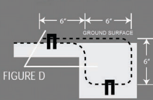
FIGURE C – PROFILE VIEW
