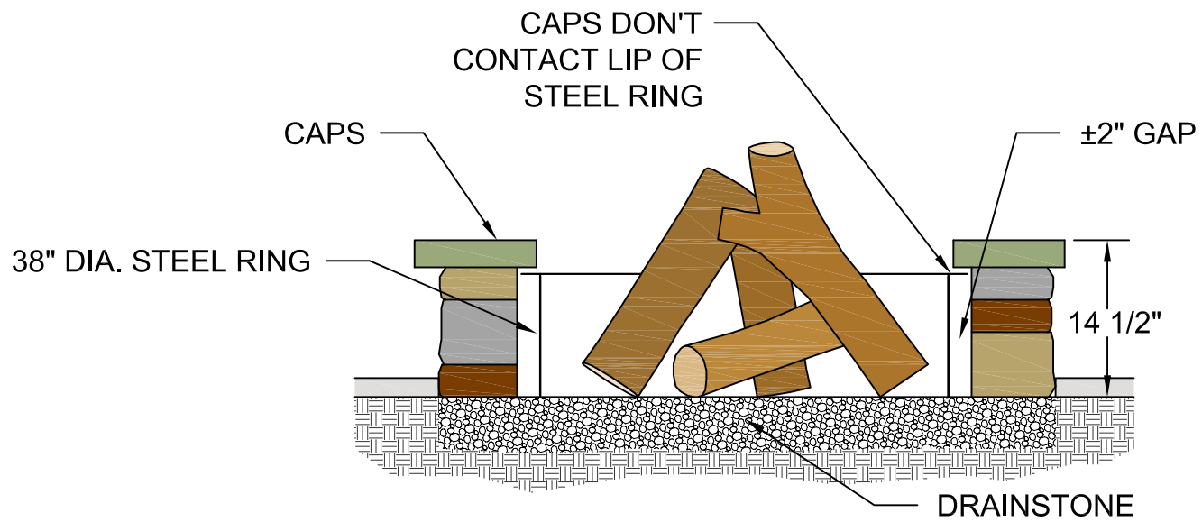
CROSS-SECTION
